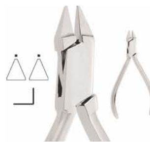
DG1-1785 Adams Plier Adams pliers for bending wire arches and bends right angles for wires up to .022 inch, .025 tip to beak. Length 13cm
